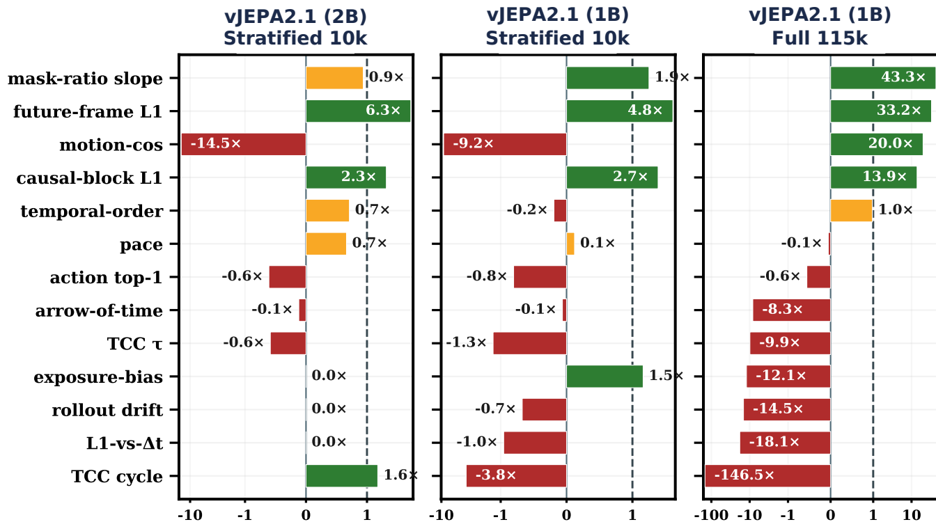
FactorJEP A vs. the best competitor, across scale: separation in 95%-CI units (rows sorted best-to-worst by the 115k panel; dashed line = the 1× separation threshold)
